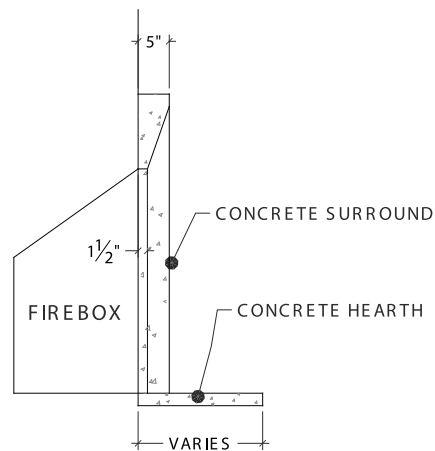
SECTION @ FIREBOX
