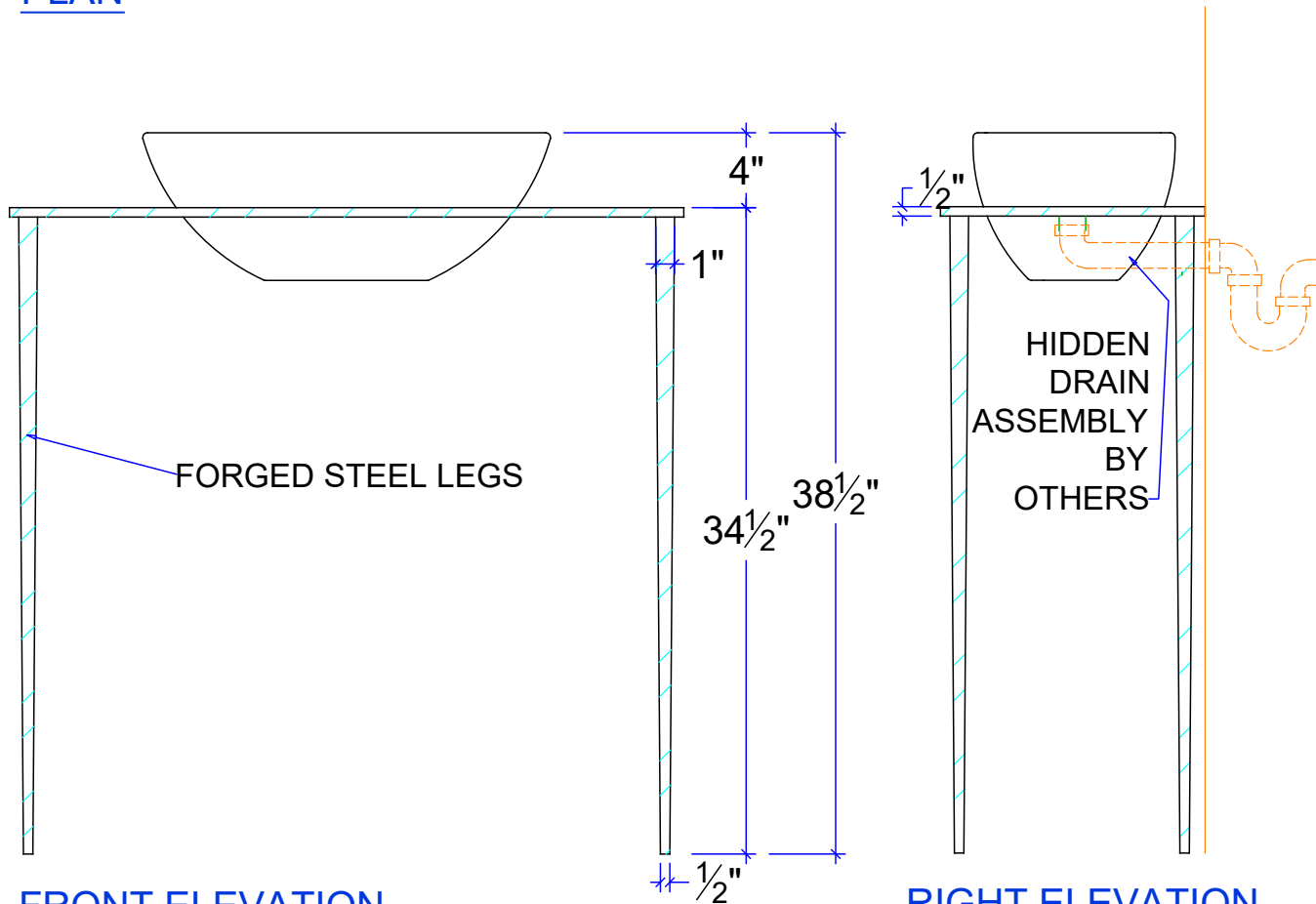
FRONT ELEVATION
