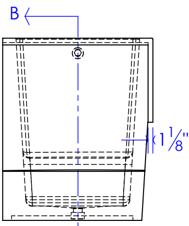
LEFT ELEVATION
