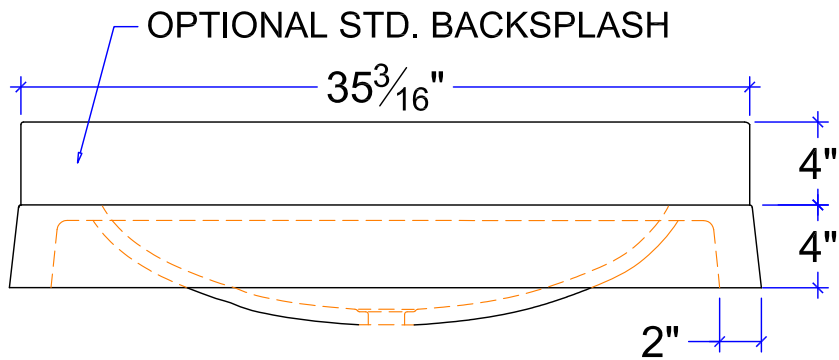
FRONT ELEVATION
