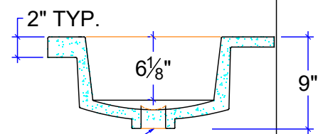
SECTION BEYOND SINK
