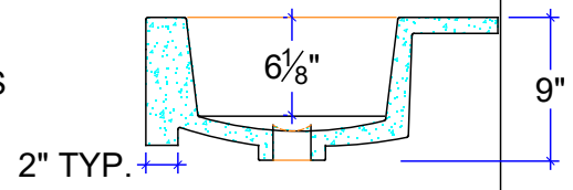
SECTION @ DRAIN
