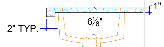
SECTION BEYOND SINK
