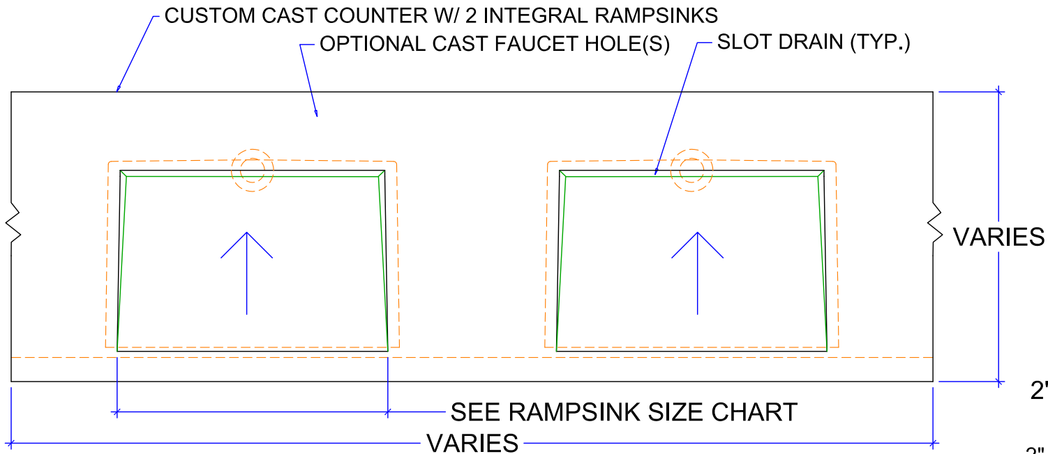
PLAN
