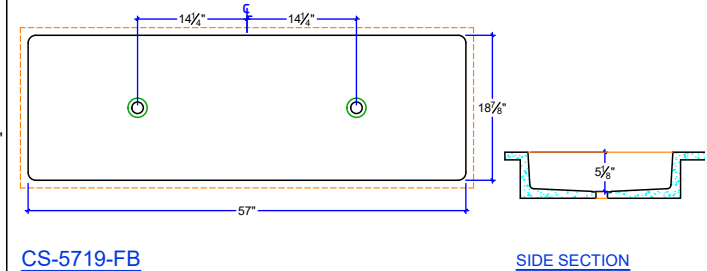
SIDE SECTION
