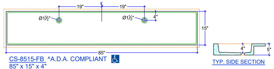
SIDE SECTION
