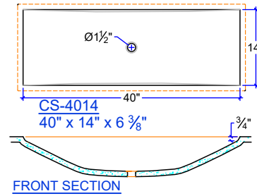
FRONT SECTION
