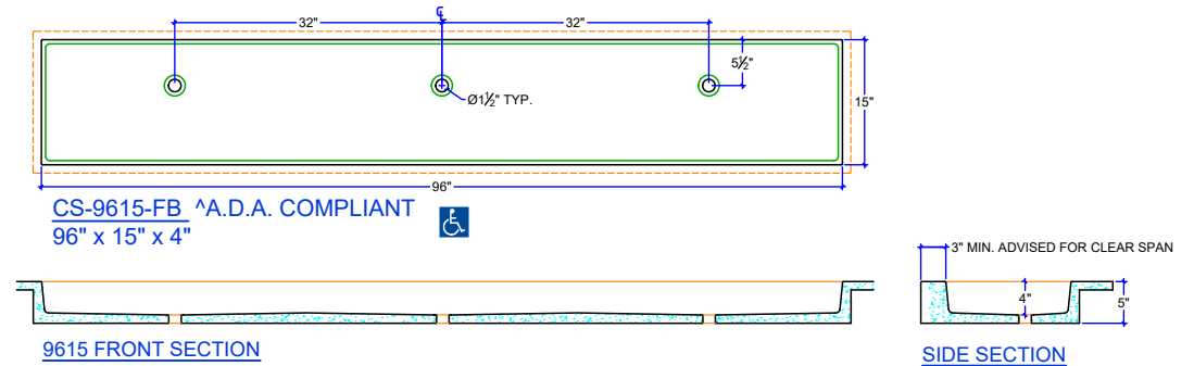
SIDE SECTION
