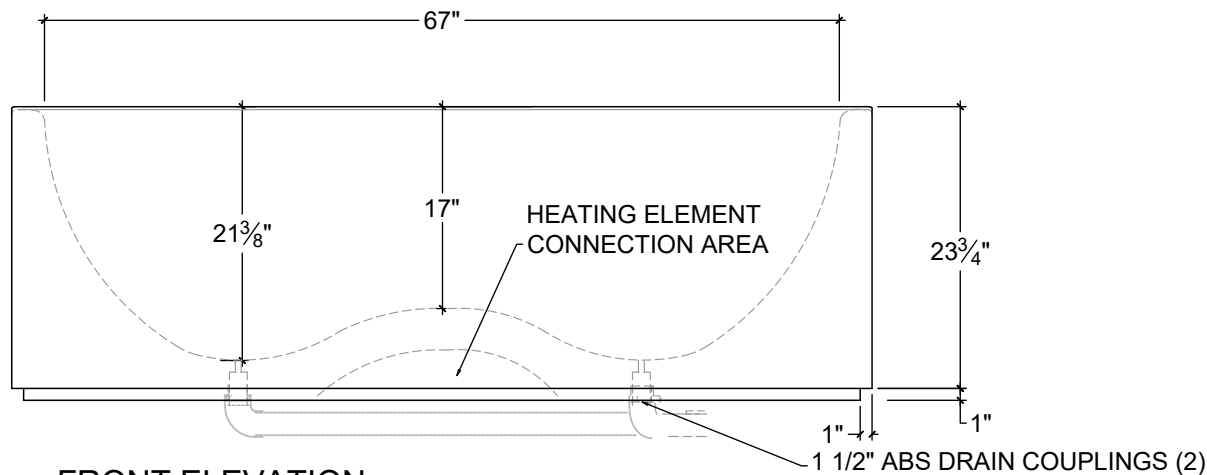
FRONT ELEVATION
