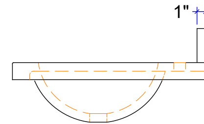
SECTION @ DRAIN
