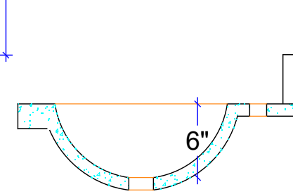
SECTION @ DRAIN
