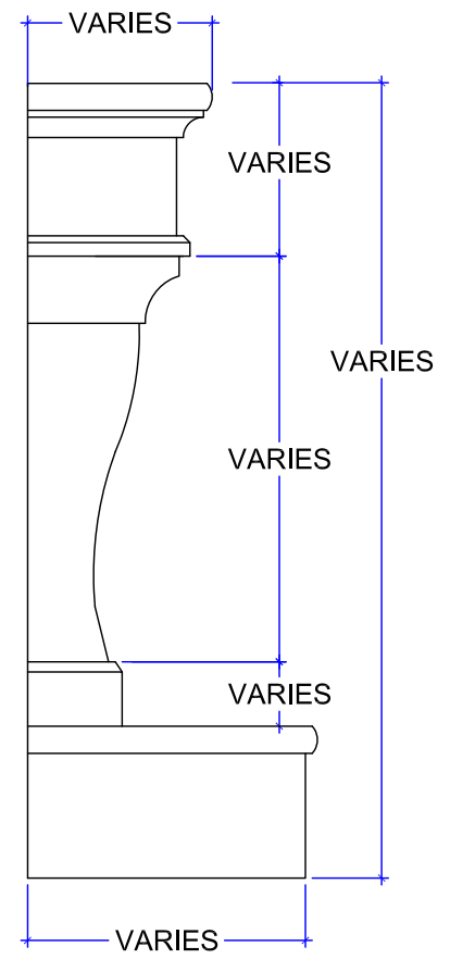
SIDE ELEVATION
