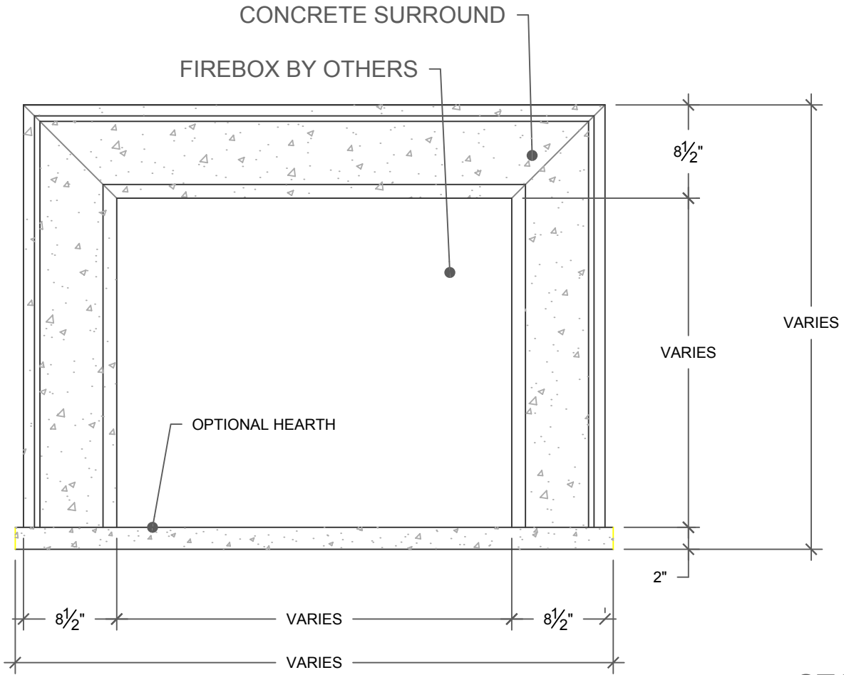
FRONT ELEVATION
