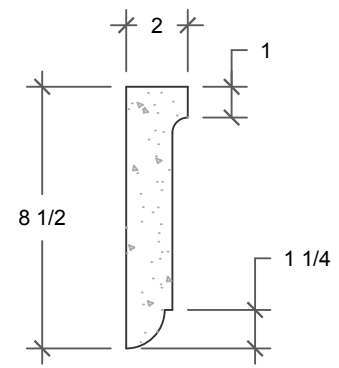
STANDARD PROFILE
