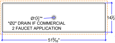
CS-5215-FB ^A.D.A. COMPLIANT (offset drain hardware req. for ADA- by others) 51.5" x 14.5" x 5"
