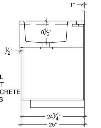
SECTION THROUGH SINK
