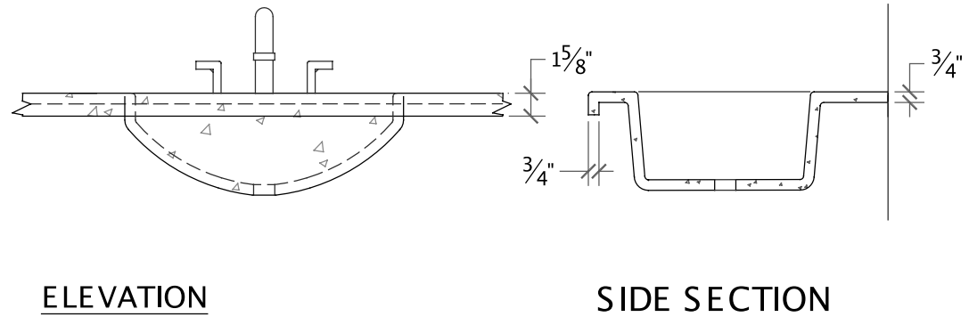
CONCRETE COUNTER W/INTEGRAL COUNTERSINK
