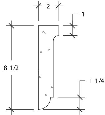
STANDARD PROFILE
