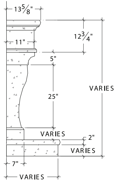
SIDE ELEVATION
