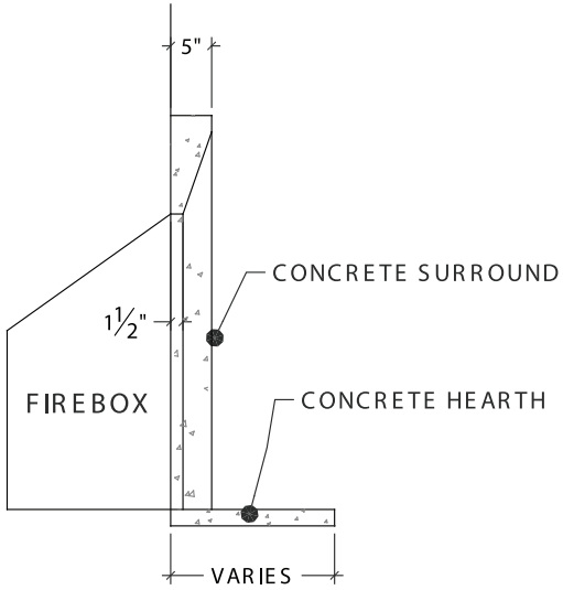
SECTION @ FIREBOX
