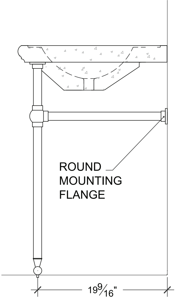
SIDE ELEVATION
