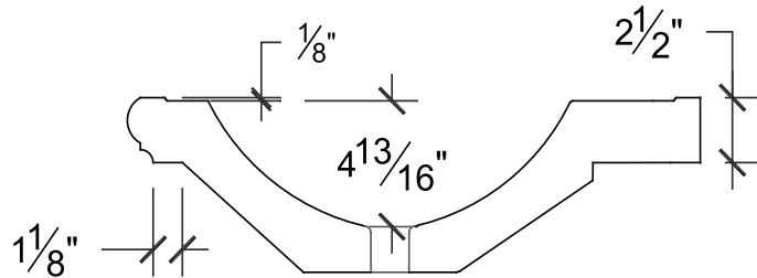
SIDE ELEVATION
