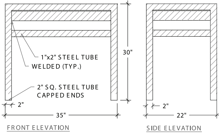
P-RAMP & P-TROUGHSINK STAND
