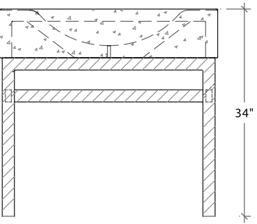
METAL STAND WITH P-WAVE
