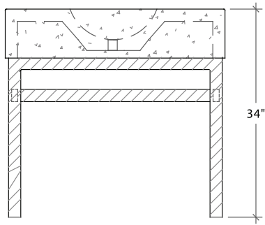
METAL STAND WITH P-COUNTERSINK
