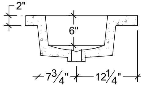
SIDE SECTION
