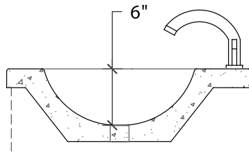
SECTION W/ 2" FRONT EDGE
