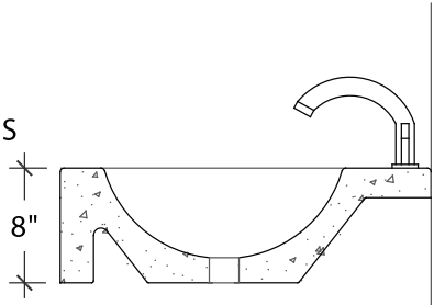
SECTION W/ 8" FRONT APRON
